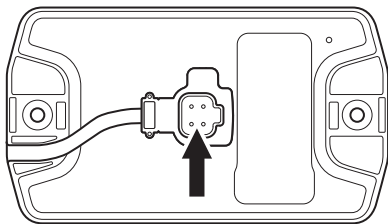
VIEW - REAR LAMP 4 PIN DT SOCKET
