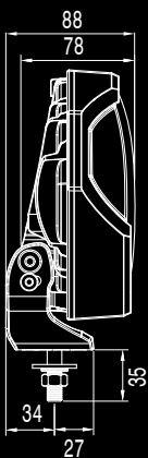
LEFT VIEW
