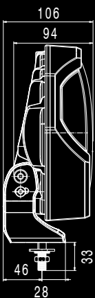
LEFT VIEW
