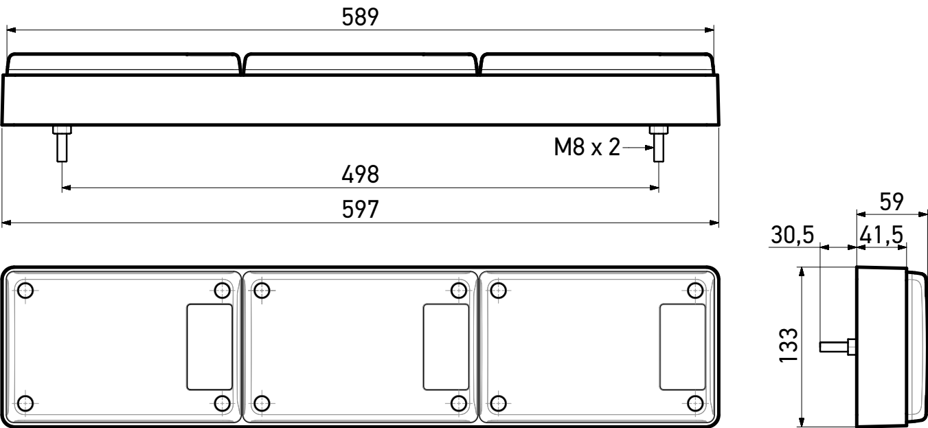
General Dimensions (in millimetres)
