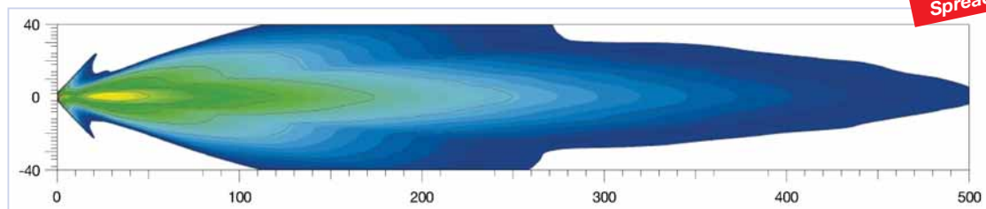
Rallye 4000 Compact Pencil Beam Distance: Recorded with single lamp. Distance in metres.
