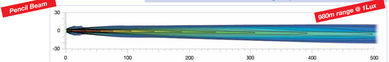
Predator Pencil Beam Distance: Recorded with single lamp. Distance in metres.
