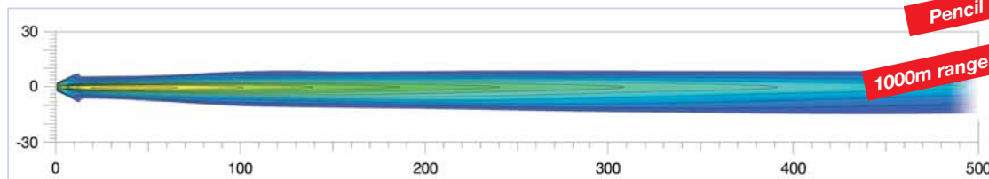
Rallye 4000 Compact Pencil Beam Distance: Recorded with single lamp. Distance in metres.
