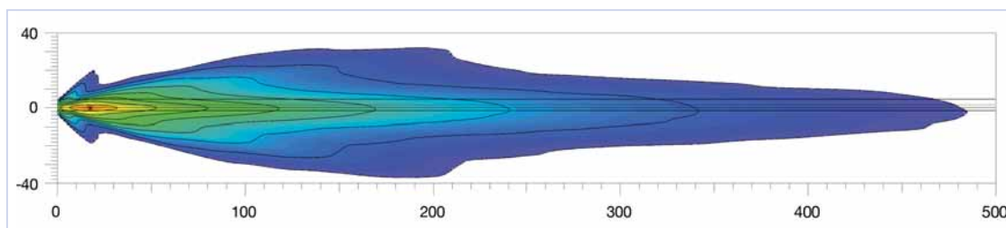
Jumbo 320 Xenon Spread Beam Distance: Recorded with single lamp. Distance in metres.
